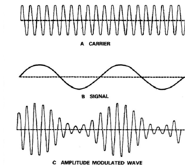
Figure 17 - AM modulation
